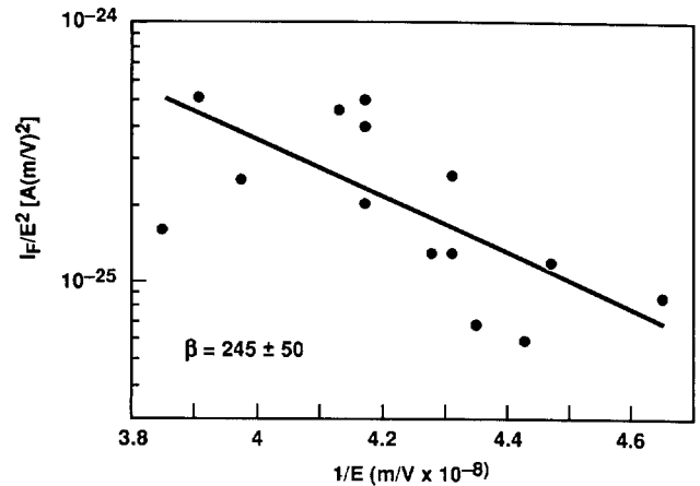
FIG. 3. Fowler-Nordheim plot for a functioning gyroscope.
