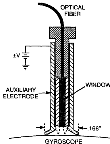
FIG. 5. Schematic representation of the UV charge control assembly with optical fiber.
