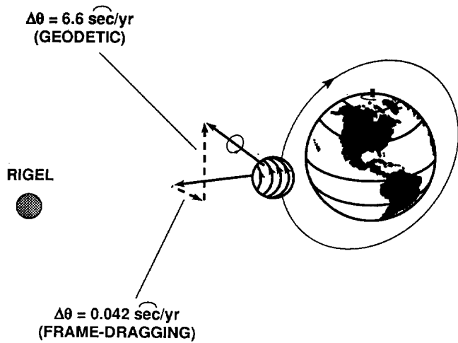
FIG. 1. GP-B geodesic and frame-dragging precessions predicted by general relativity.
