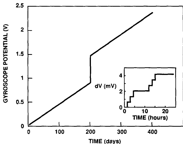
FIG. 4. Calculated gyroscope charging due to trapped and solar flare protons. The orbital period is 1.5 h.
